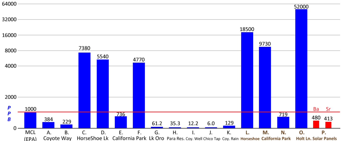
Aluminum in Chico Water in Parts Per Billion — Samples should be less than 1 PPB Nominal
